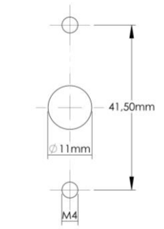
VERTICAL mounting
