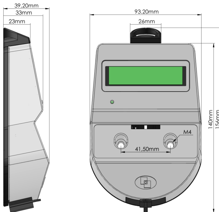
STANDARD mounting
