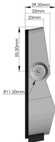
STANDARD mounting
