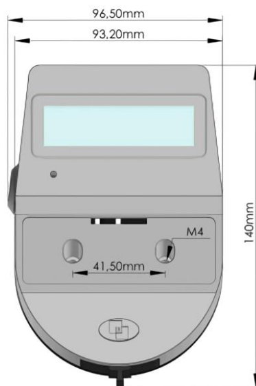
VERTICAL mounting
